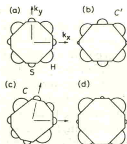
Fig. 7. Schematic representation of the Brillouin zone and overlap electron populations of aluminium in various strains states
